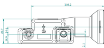
O-LNB
