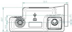
O-LNB C120
